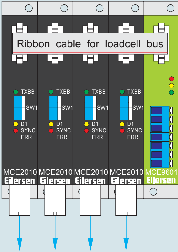
BNC connectors for load cells
